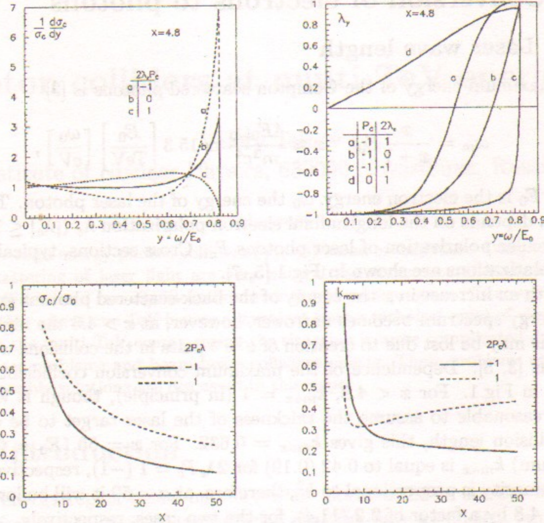
Figure 1: From left-upper corner: a) spectra of Compton scattered photons; b) helicity of scattered photons; c) Compton cross section vs x in the case of linear Compton scattering; d) maximum conversion coefficient (due to e^+e^- pairs) vs x .
