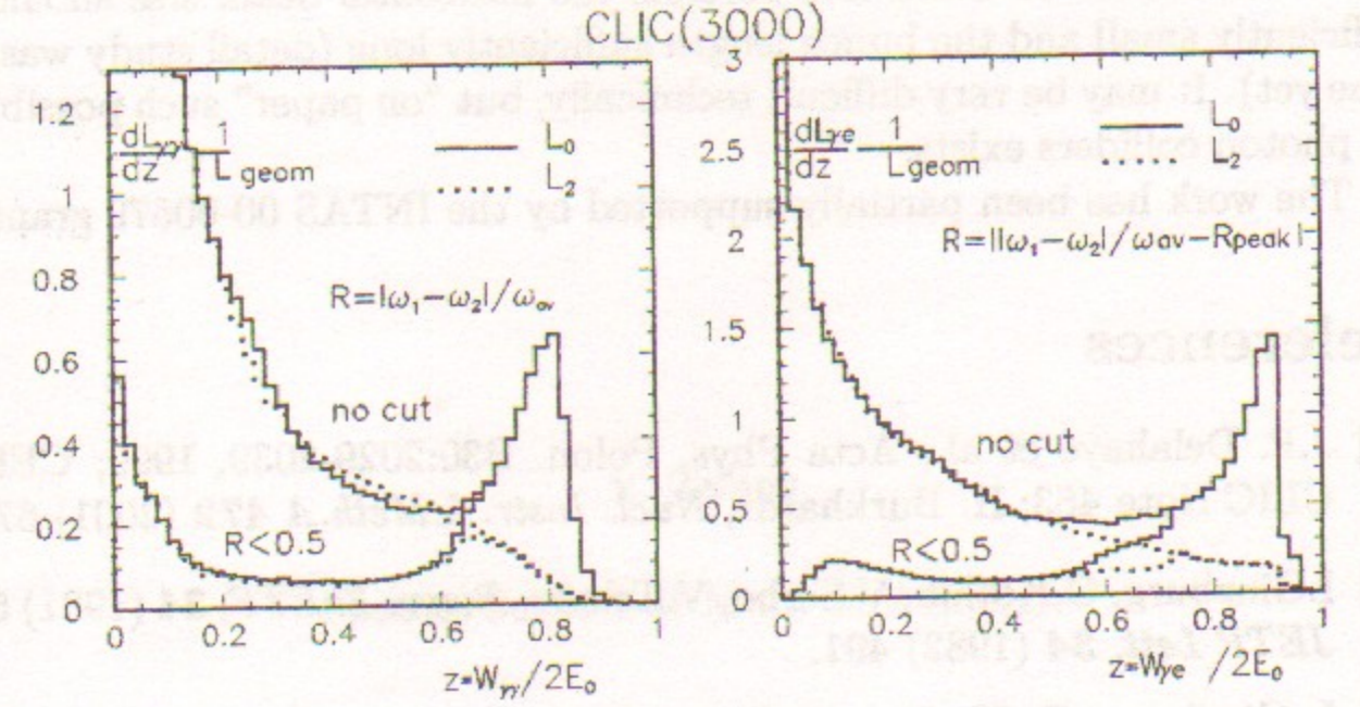
Figure 2: \gamma\gamma and \gamma e Luminosity spectra at CLIC(3000).
