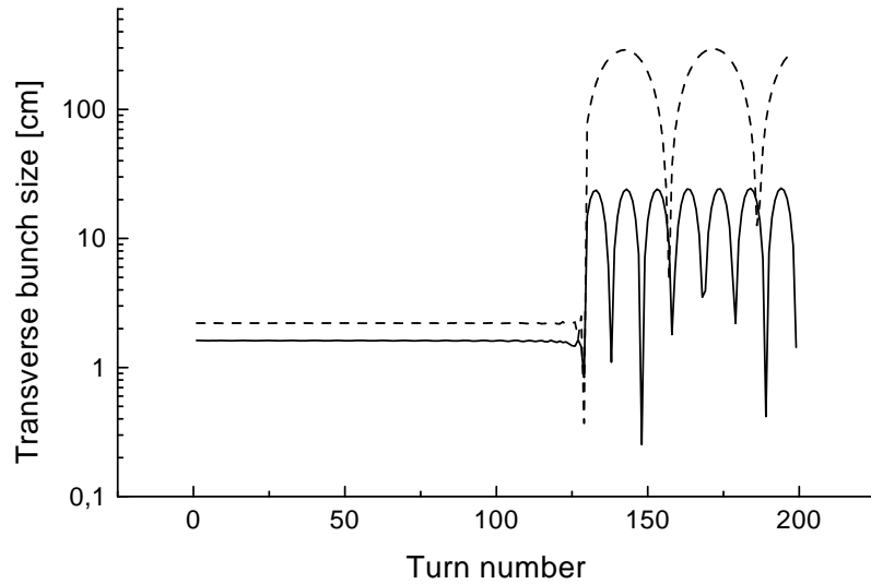
Figure 5.7: Dependences of the vertical (solid line) and horizontal (dashed line) beam sizes on the turn number. Number of particles 10^{13} of U^{4+} ions, W = 125 MeV/u, V_0 = 1.211 MV during first 100 turns, \epsilon = 10 mmmrad, \sigma_{in} = 600 m, (\sigma_\delta)_{in} = 3 \times 10^{-6} .
