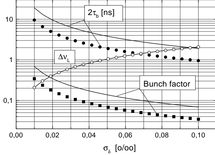
Figure 2.10: Dependencies of the bunch length ( 2\tau_b ), bunching factor ( B = 2h\tau_b/T_0 ) and of the Laslett tune shift in cases of longitudinal phase space matching on the momentum spread of injected bunches. Solid lines -W = 5 MeV/u, h = 1400 , symbols -W = 10 MeV/u, h = 994 .
