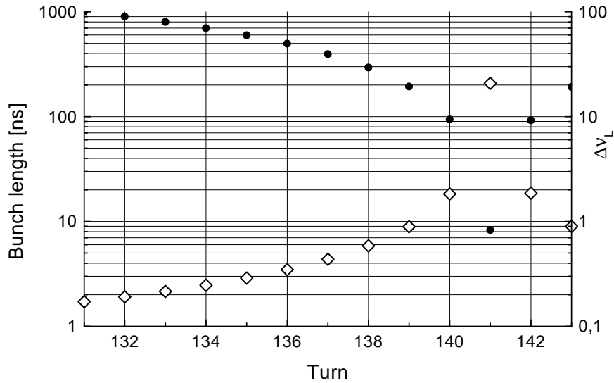
Figure 4.21: Dependence of the bunch length (full circles) and of the Laslett tune shift (open diamonds) on the turn number. N = 10^{13} of U^{4+} ions, W = 125 MeV/u, V_0 = 1.131 MV, k = 10 , \sigma_{in} = 600 m, \delta_{in} = 3 \times 10^{-6} , one RF-station/turn, a drift space between RF-stations is divided by 4800 steps.
