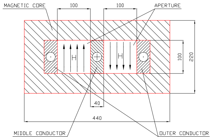
Figure 5.6: Schematic (input) cross section of the two-aperture bending magnet (BM).
