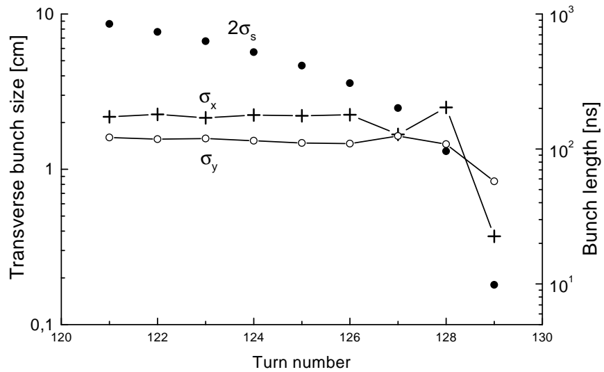
Figure 5.8: The last 10 turns of the bunch compression for parameters same as in Fig.5.7.
