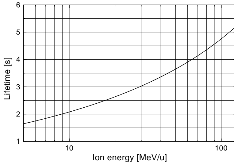
Figure 2.2: Dependence of the lifetime on the \text{U}^{4+} ion energy. P=0.01 nTorr, the gas mixture is assumed to be 77% \text{H}_2 +20% \text{N}_2 +3%Ar.
