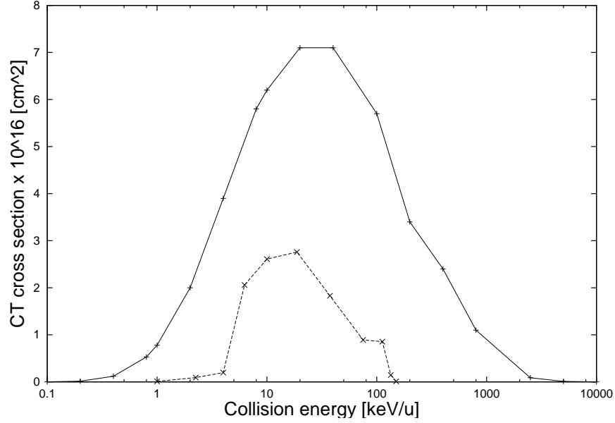
Figure B.1: Dependence of the charge transfer cross section for collisions of the U^{4+} ions on their collision energy. Crosses – data from Table B.2, x – data from the Table B.1.
