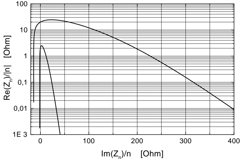
Figure 4.2: Stability diagram for coherent oscillations of the coasting beam after debunching. The beam contains 10^{13} of ions U^{4+} , kinetic energy 125 MeV/u, slip factor 0.77, outer curve -\sigma_\delta = 3.5 \times 10^{-5} , inner curve -\sigma_\delta = 1 \times 10^{-5} . Only upper half of the diagrams are shown in the graph.
