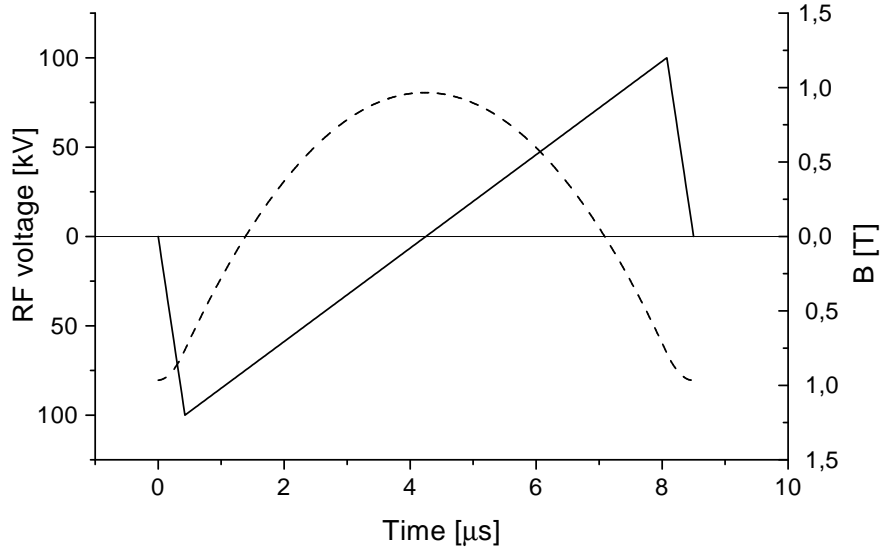
Figure 6.6: The shape of one period of the specific sawtooth RF-voltage per one meter of the magnetic cores length (solid line) and the inductance time diagram in the permalloy during one RF-period (dashed line).
