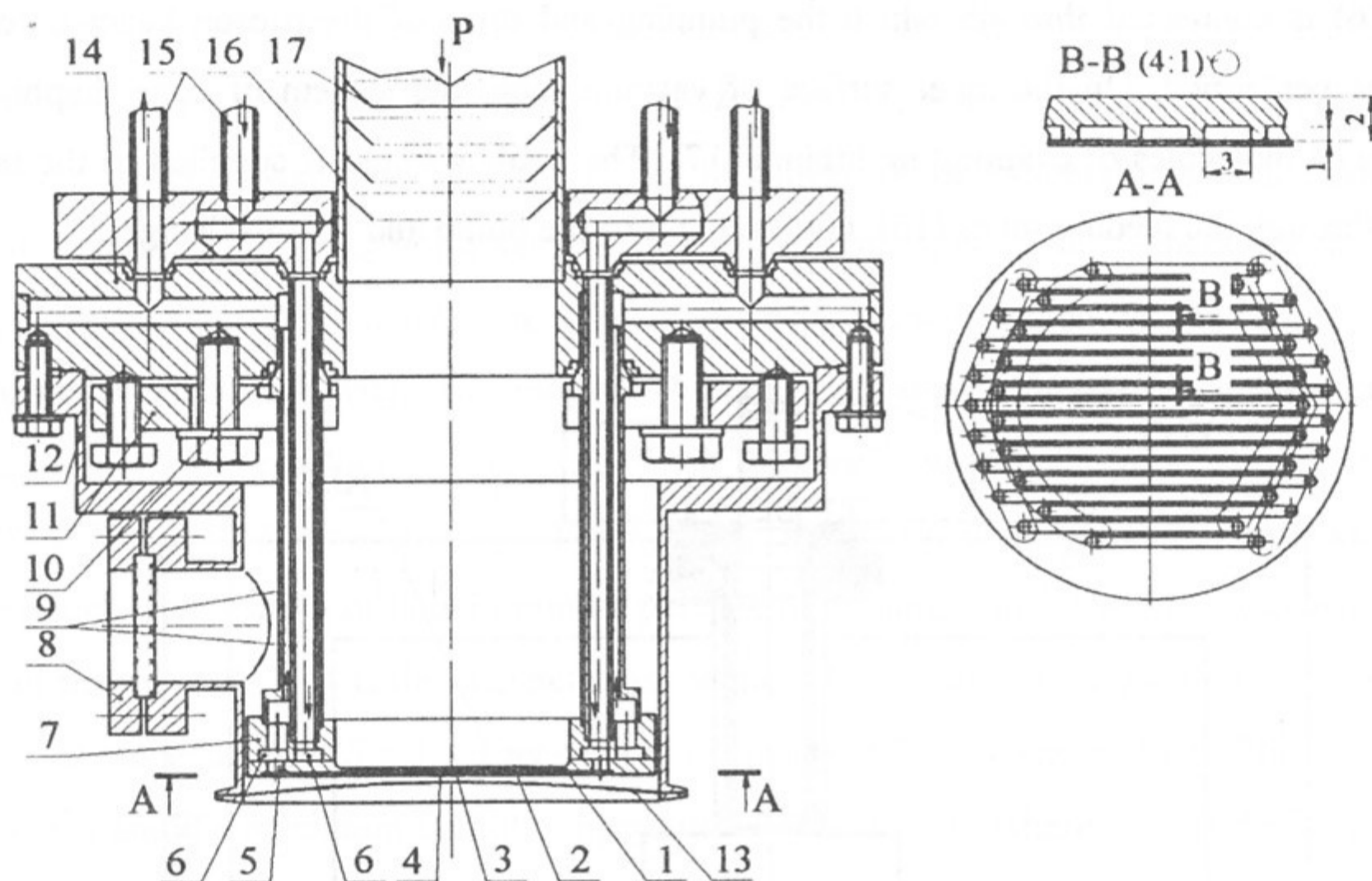
Figure 18. Neutron generating lithium target . 1 - tungsten disk; 2 - lithium layer; 3 - cooling channels; 4 - tantalum foil; 5 - feeding holes; 6 - collector cavities; 7 - tantalum ring; 8 - observing window; 9 - feeding coaxial tubes; 10 - copper packings; 11 - lever clamps; 12 - vacuum chamber; 13 - molybdenum foil; 14 - body; 15 - heat carrier feeding tubes; 16 - vacuum chamber; 17 - cone caters of lithium vapors.
