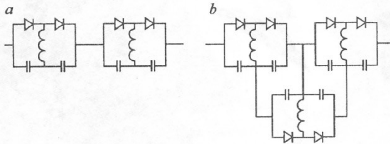
Figure 14. ELV rectifying section circuit and means of their connection.
