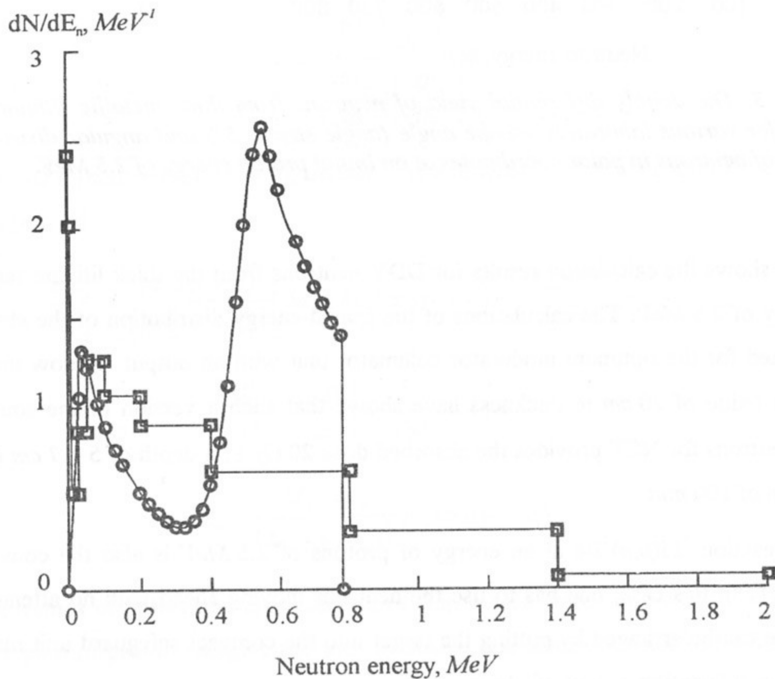
Figure 4. Energy neutrons spectrum for {}^7\text{Li}(p,n){}^7\text{Be} reaction at 0^\circ laboratory angle and initial proton energy 2.5\text{ MeV} and neutrons energy distribution for BR-10 reactors medical neutron beam B-3.
