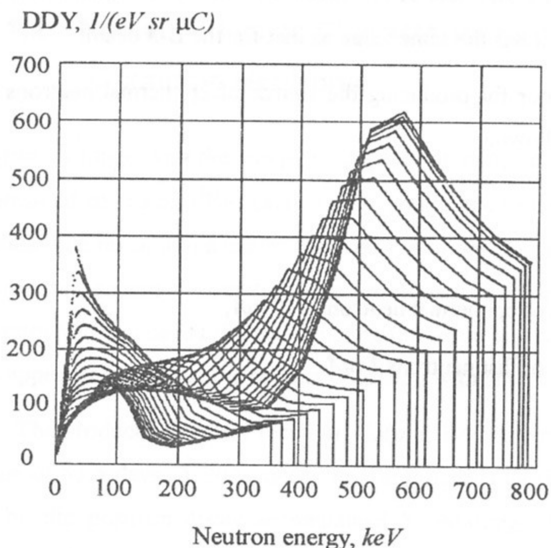
Figure 3. The doubly differential yield of neutrons from thick metallic lithium target for various laboratory escape angle (angle step is 5^\circ ) and angular distribution of neutrons in polar coordinates at an initial proton energy of 2.5 MeV.
