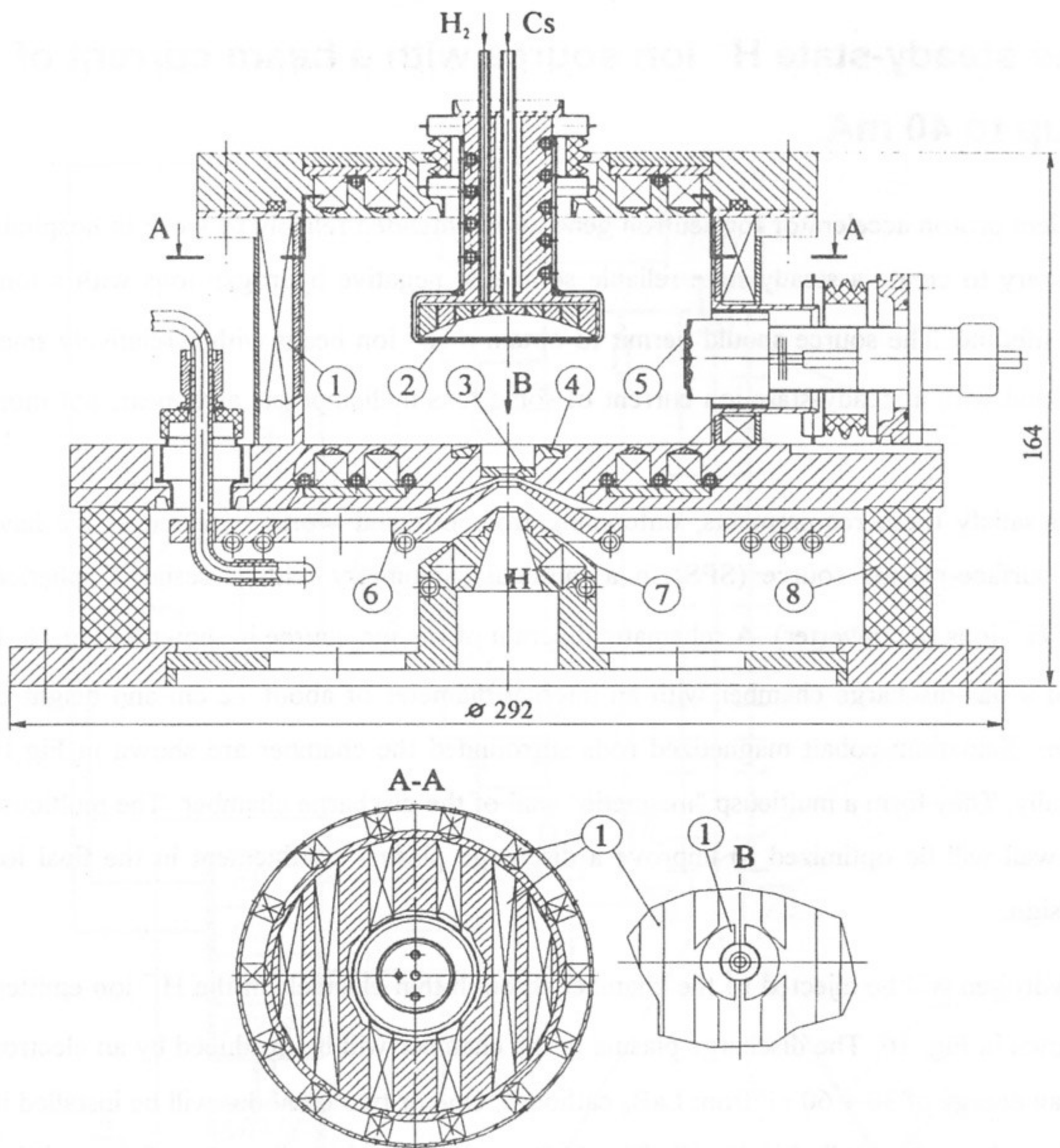
Figure 16. H^- ion source. 1 - «magnetic» wall of gas-discharge chamber, 2 - emitter of H^- ions, 3 - plasma electrode with outlet hole, 4 - magnetic filter of electrons, 5 - LaB_6 cathode, 6 - extractor, 7 - accelerating electrode, 8 - 30 kV main insulator.
