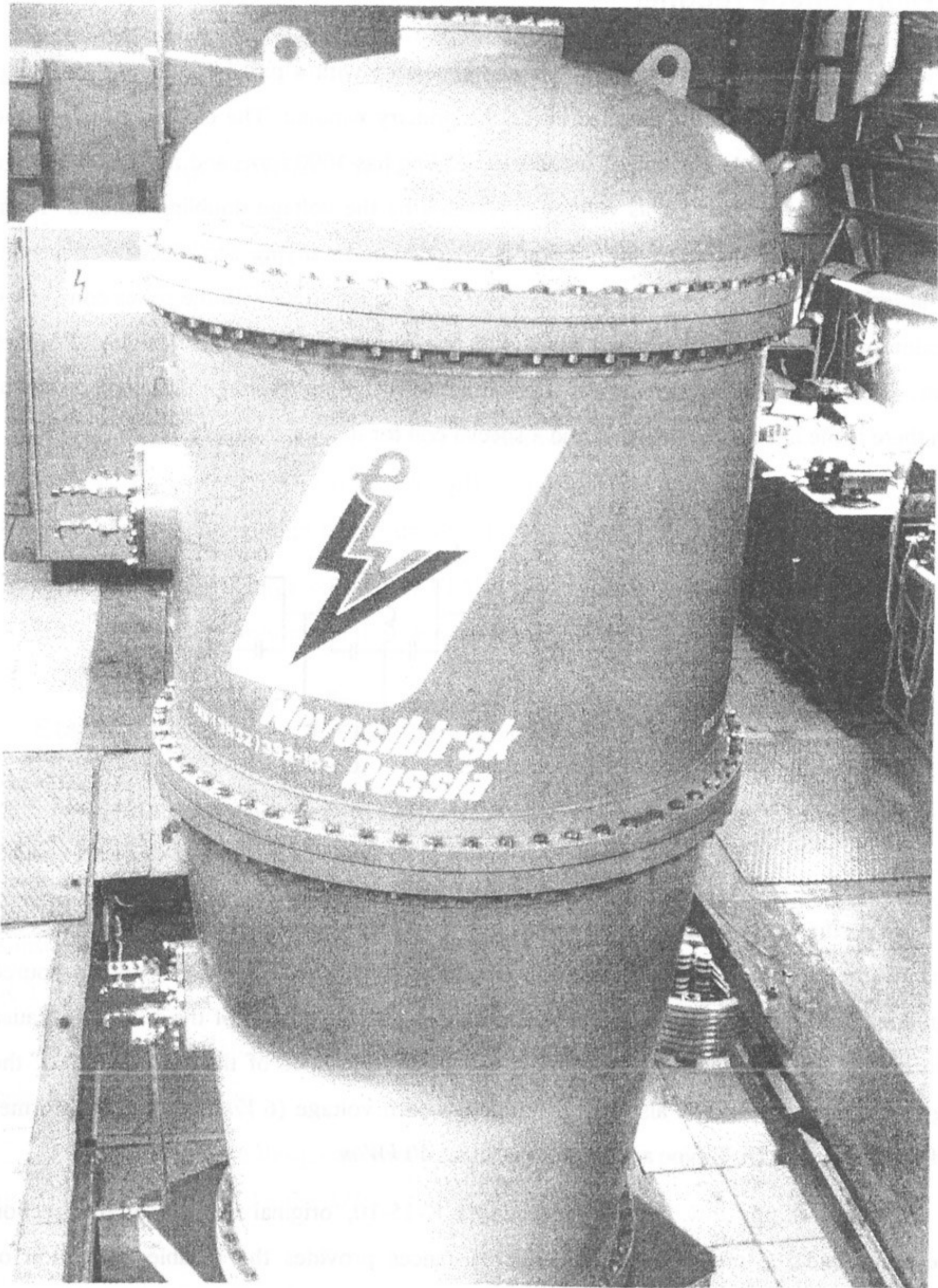
Figure 13. Photo of the accelerator ELV-8.
