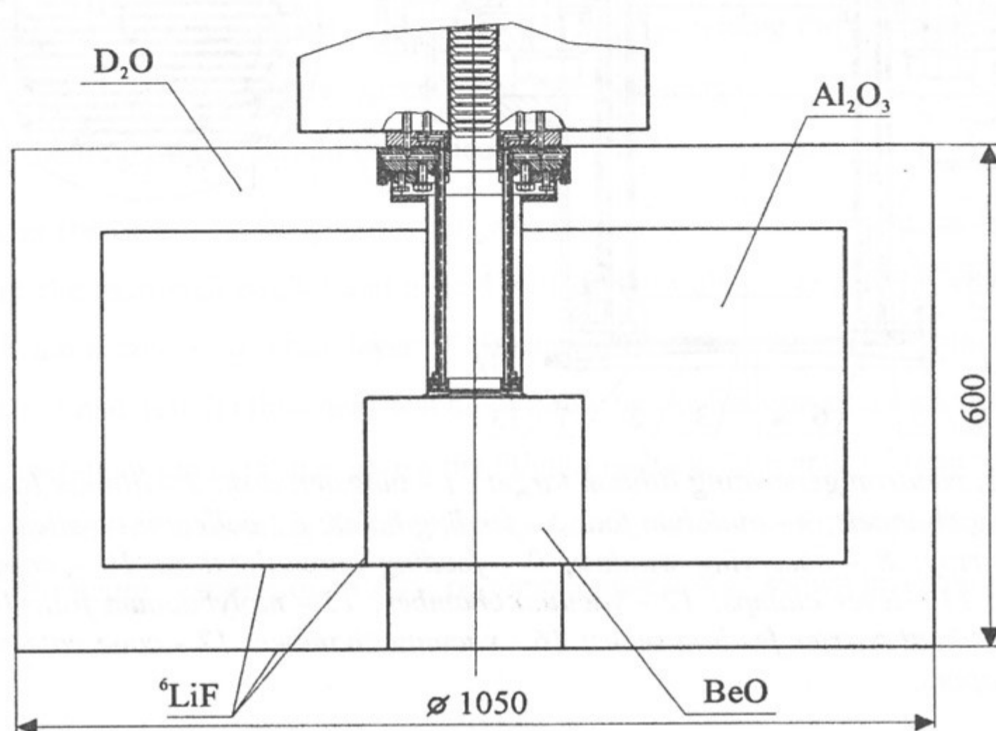
Figure 19. Target with moderator and reflector.
