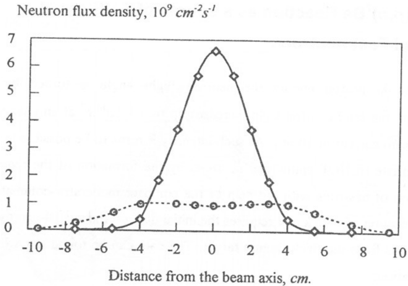
Figure 2. The radial distributions of neutron flux in planes remote from the target at distances 3 cm ( \diamond ) and 10 cm ( \circ ) for incident proton energy of 1896 keV and beam current of 10 mA.
