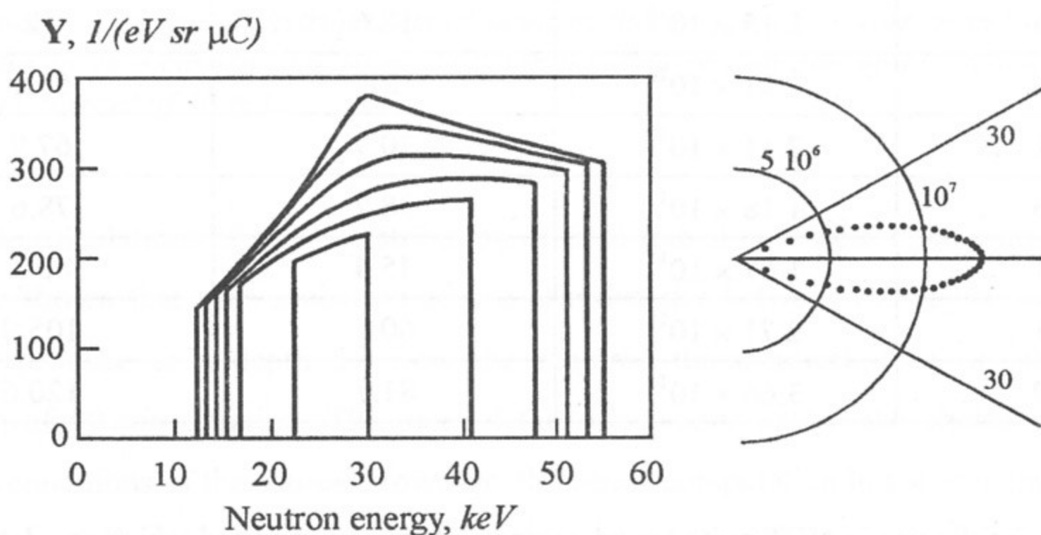
Figure 1: The doubly differentiated yield of neutrons from thick metallic lithium target for various laboratory escape angle (angle step is 5^\circ ) and angular distribution of neutrons in polar coordinates at an initial proton energy of 1886 \text{ keV} .
