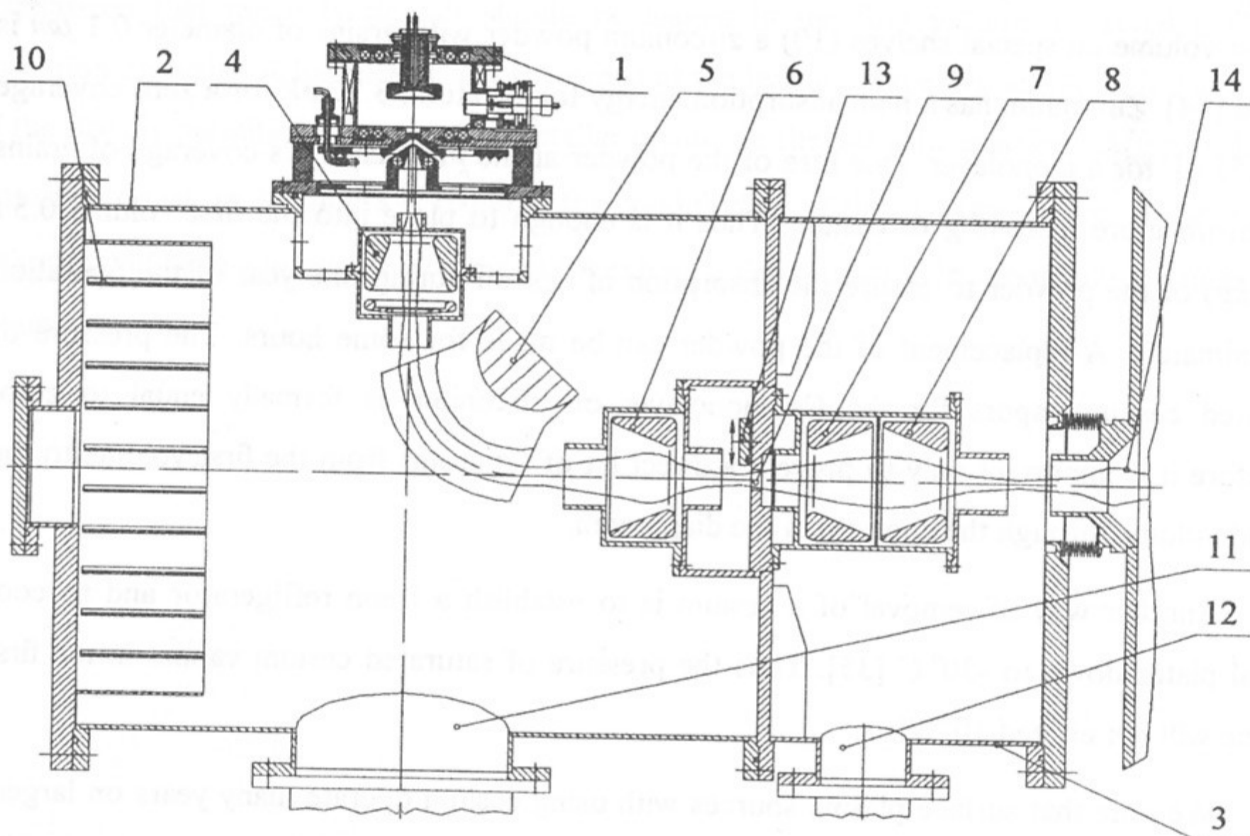
Figure 17. Chamber of H^- ion source. 1 - H^- ion source, 2 - 1 st volume, 3 - 2 nd volume, 4, 6, 7, 8 - electrostatic lenses, 5 - separating (bending) magnet, 9 - inter-volume aperture, 10 - shelves with zirconium powder, 11, 12 - holes for turbomolecular pumps, 13 - vacuum valve, 14 - entrance into tandem accelerator.
