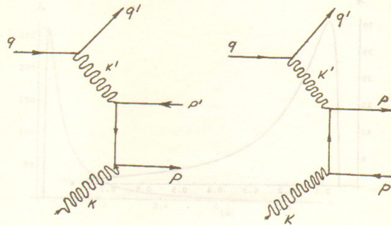
Fig.4 Diagrams of direct electroproduction of electron-positron pair.
