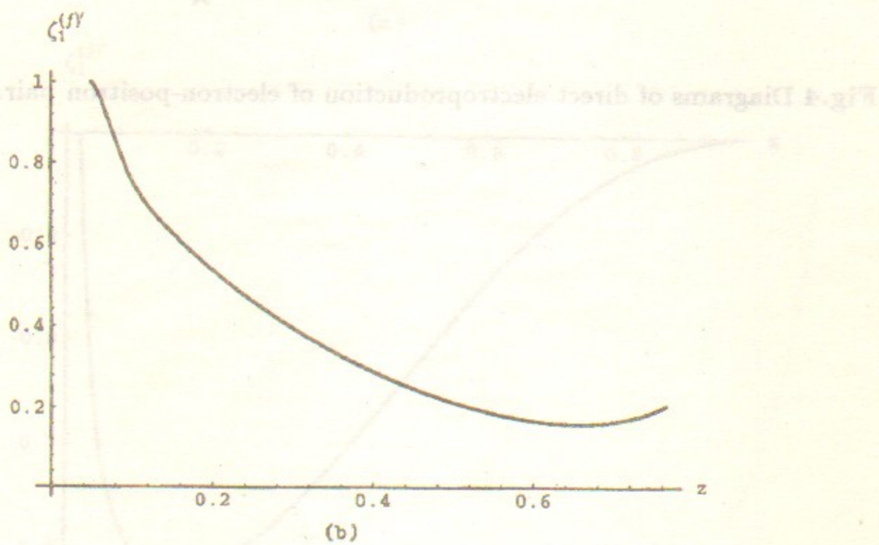
Fig.5 Characteristics of the direct electroproduction process for \lambda = 20 . The spectral distributions of the probability of direct electroproduction process for unpolarized particles and photons in units \frac{\alpha^3 \ln \lambda}{m^2 \lambda} (the term J_0 in eq.(20)) (a). Longitudinal polarization of the created positrons plotted vs z for \xi_{c2} = 1 (b).
