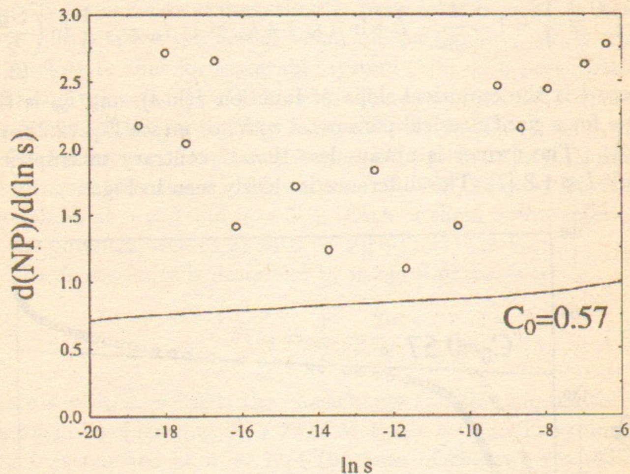
Figure 2: Derivative of the distribution function in Fig.1. Solid line shows dependence (3.6) with the same fitting parameter C_0 = 0.57 .
