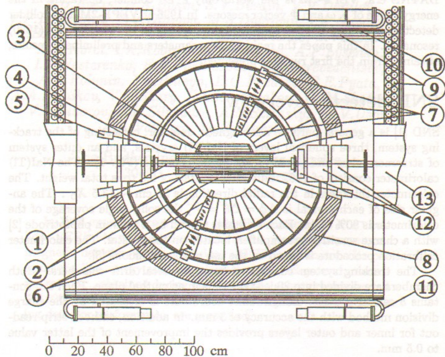
Figure 1: Detector SND — view transverse to the beam; 1—beam pipe, 2—drift chambers, 3—scintillation counters, 4—fiber lightguides, 5—PMTs, 6—NaI(Tl) counters, 7—vacuum phototriodes, 8—iron absorber, 9—streamer tubes, 10—1 cm iron plates, 11—scintillation counters, 12—magnetic lenses, 13—bending magnets
