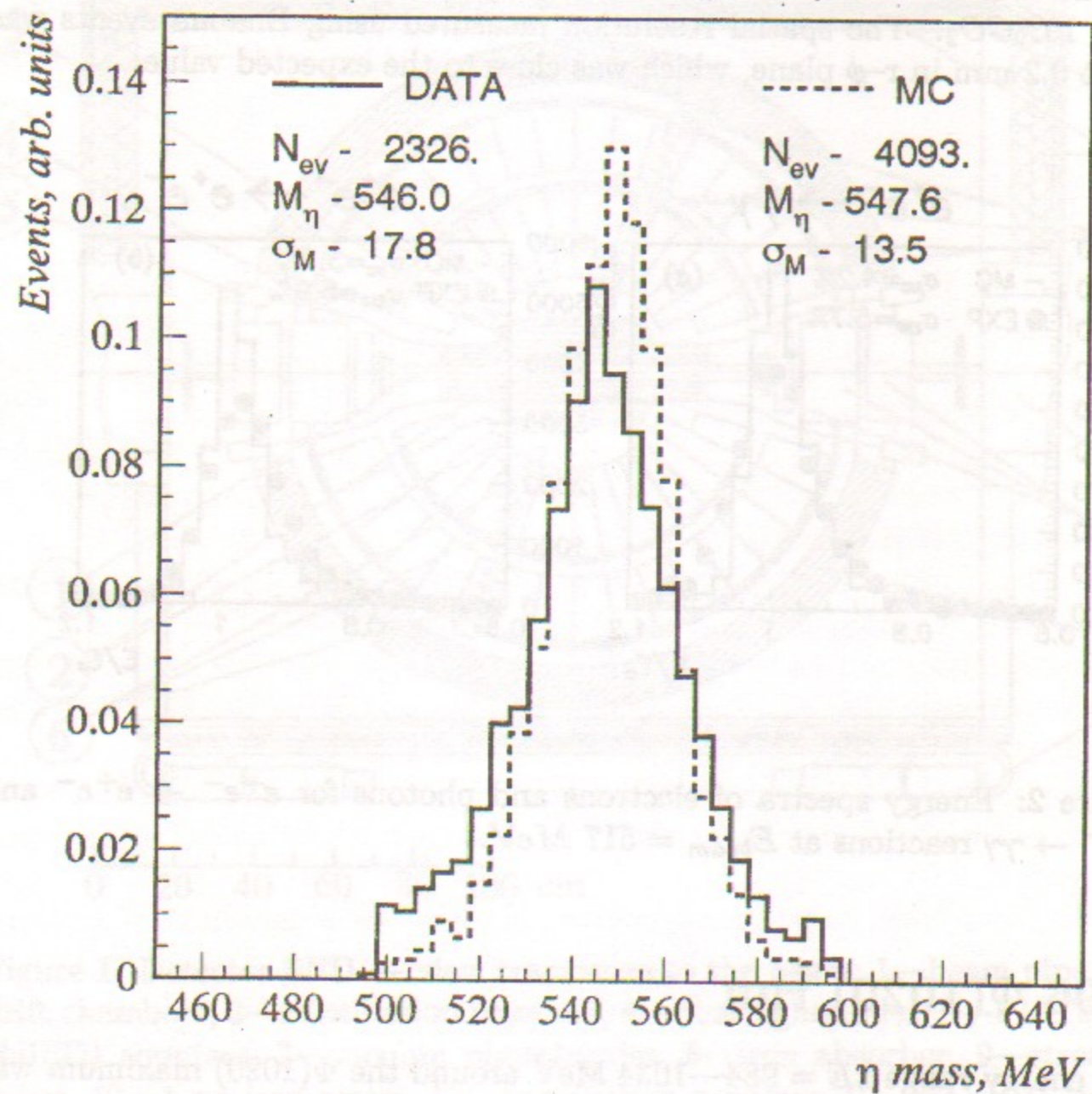
Figure 3: Effective mass spectrum of two photons for e^+e^- \rightarrow \eta\gamma \rightarrow 3\gamma reaction.
