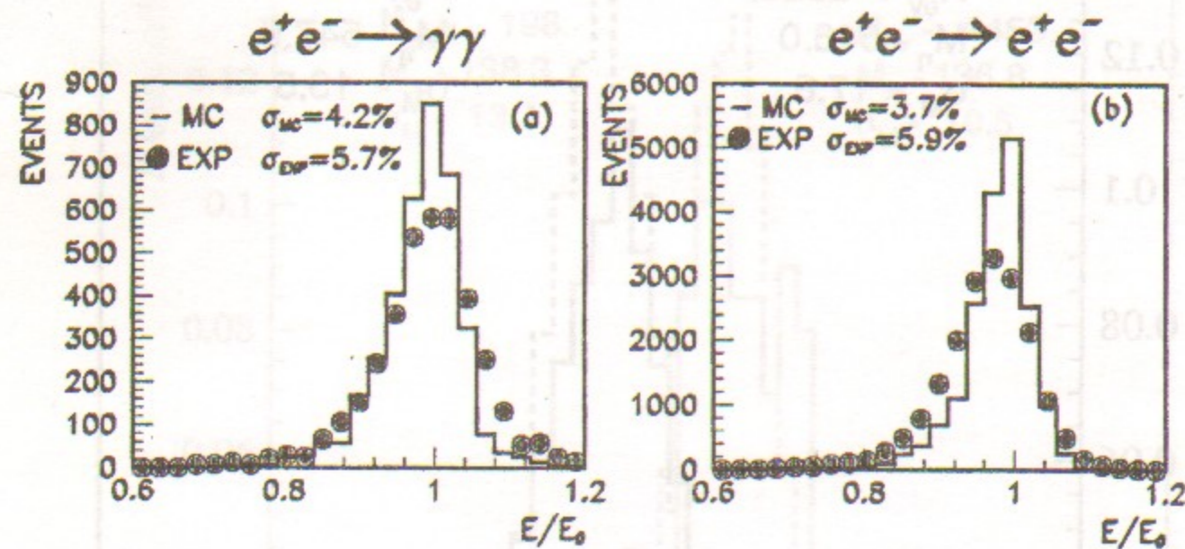
Figure 2: Energy spectra of electrons and photons for e^+e^- \rightarrow e^+e^- and e^+e^- \rightarrow \gamma\gamma reactions at E_{beam} = 517 MeV.
