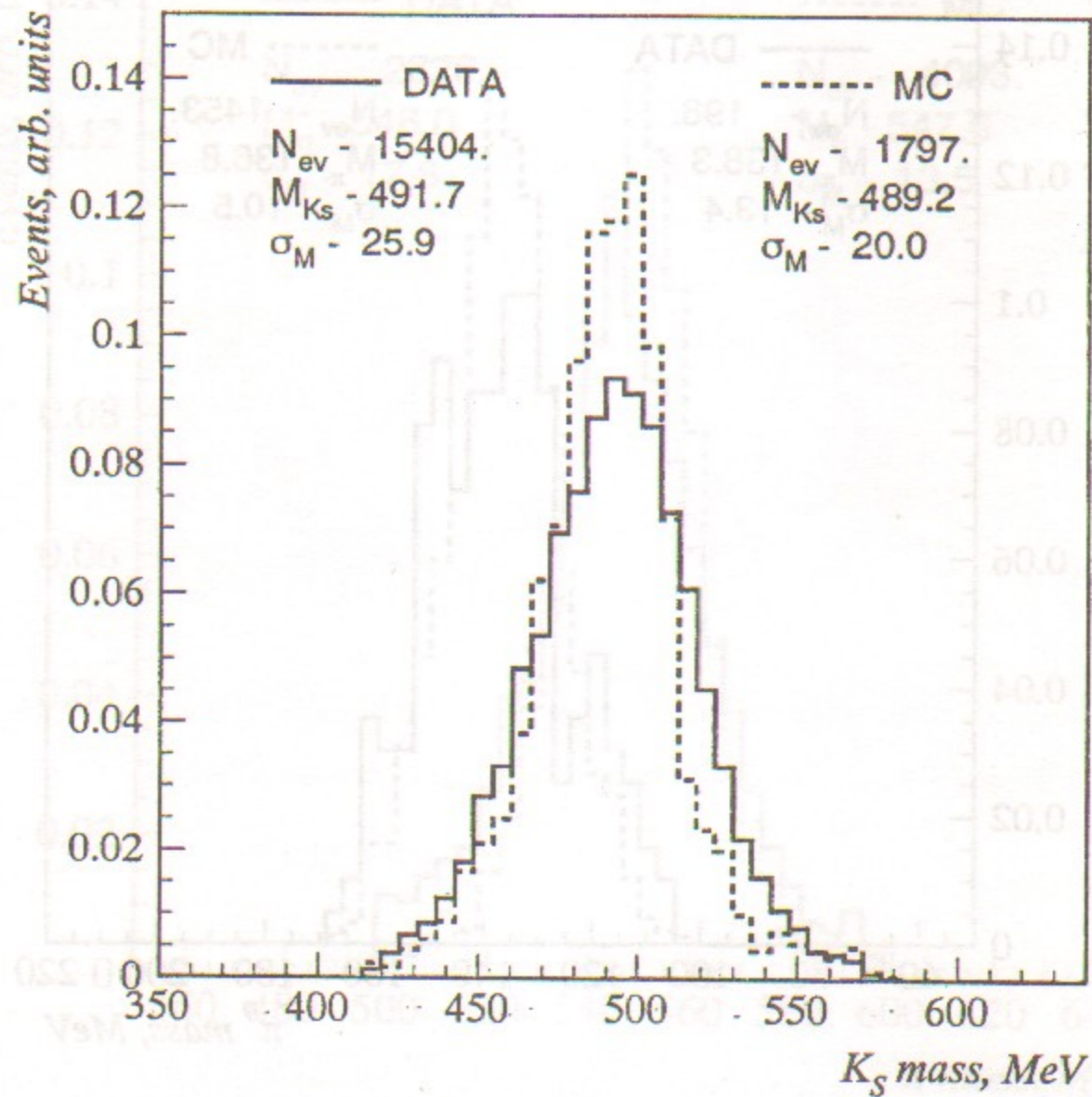
Figure 5: Effective mass spectrum of four photons for K_S \rightarrow 2\pi^0 decay.
