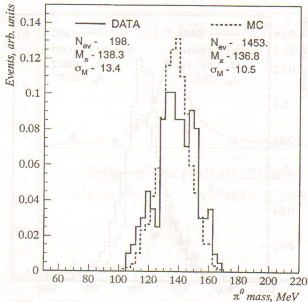
Figure 4: Effective mass spectrum of two photons for e^+e^- \rightarrow \pi^0\gamma \rightarrow 3\gamma reaction.
