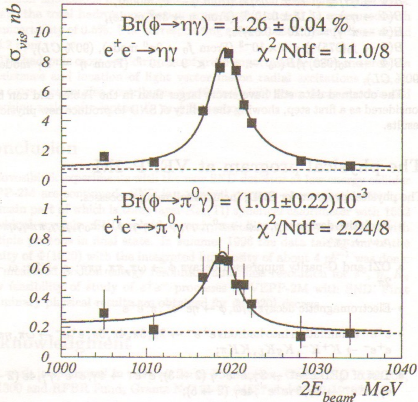
Figure 6: Visible cross section of e^+e^- \rightarrow \eta\gamma and e^+e^- \rightarrow \pi^0\gamma reactions.
