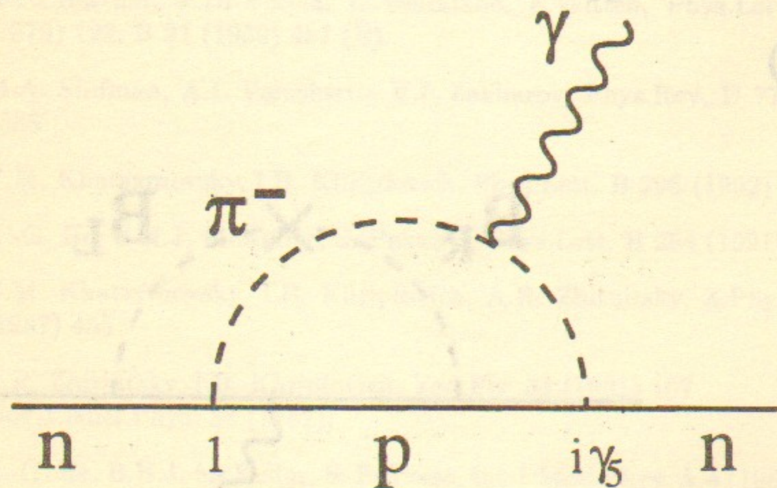
Fig. 3. Chiral contribution to the neutron EDM. \pi NN vertices 1 and i\gamma_5 refer to the CP -odd and usual strong interactions, respectively.
