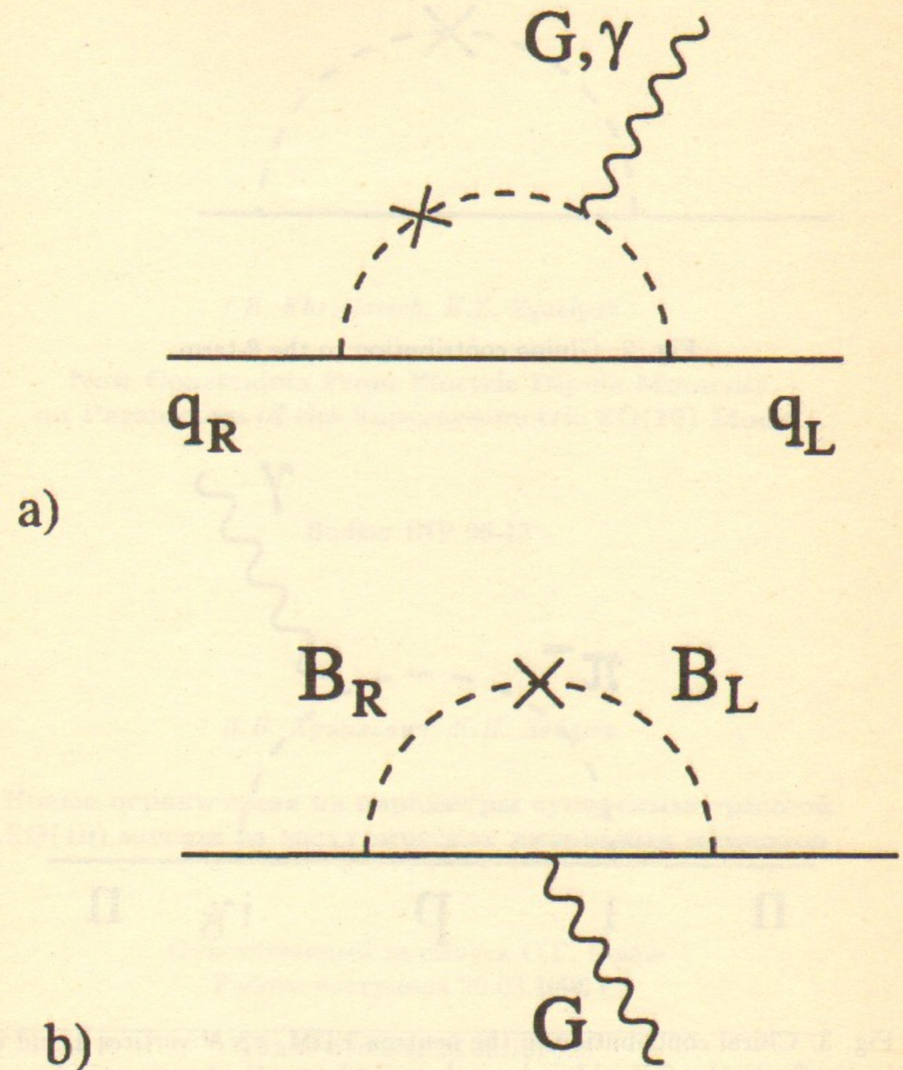
Fig. 1. Gluino contributions to quark dipole moments. B_{L(R)} denotes the left(right)-handed b -squark.
