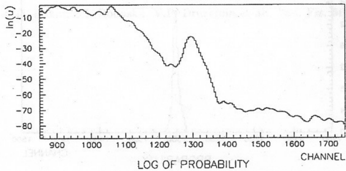
Fig.2. Invariant probability distribution for peak + background, m=3 .
