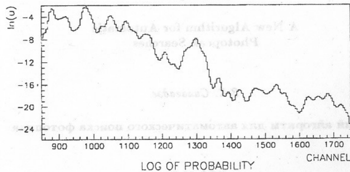
Fig.3. The same as on Fig.2 for low statistics.
