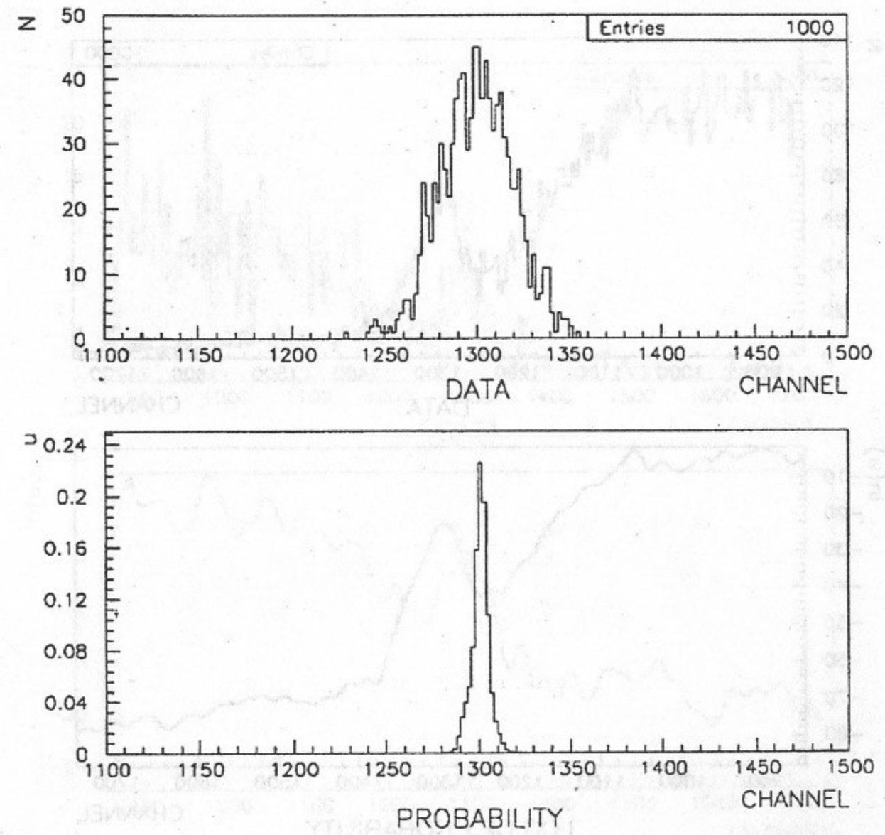
Fig.1. Invariant probability distribution u(i) for single gaussian peak, m=3 .
