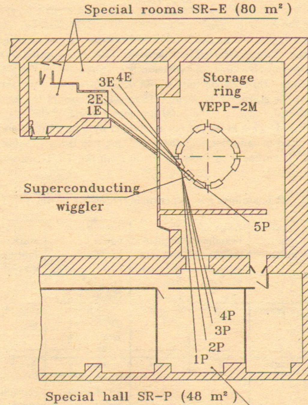
Fig. 1. Layout of the VEPP-2M facility.
