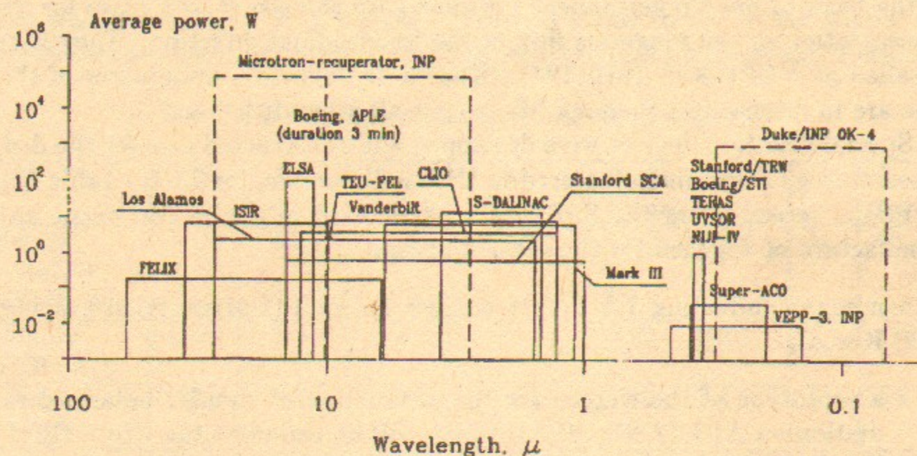
Fig. 8. Status of creating FEL in the world.
