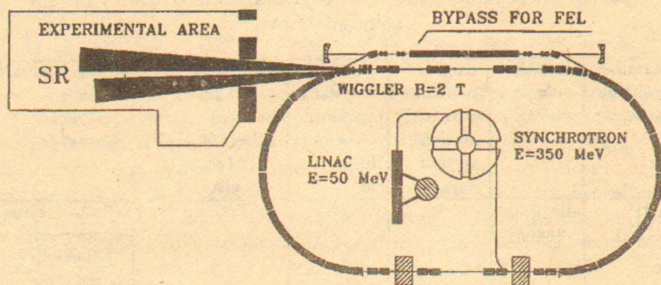
Fig. 2. Layout of the VEPP-3 facility.
