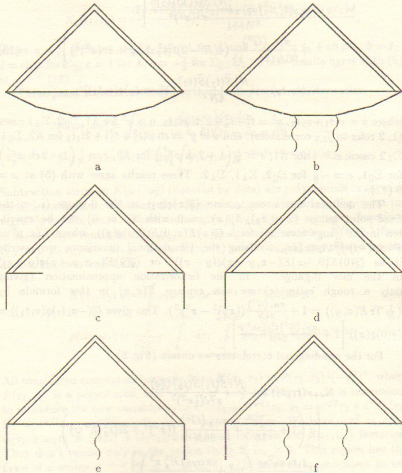
Figure 5: Three-point correlator
