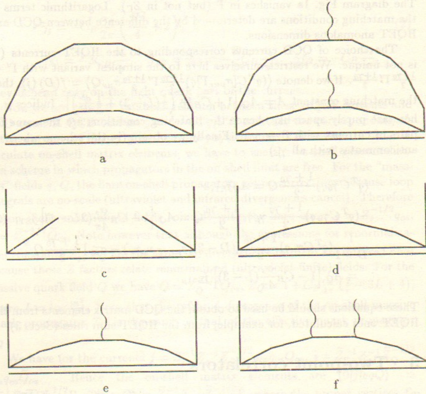
Figure 2: Two-point correlator
