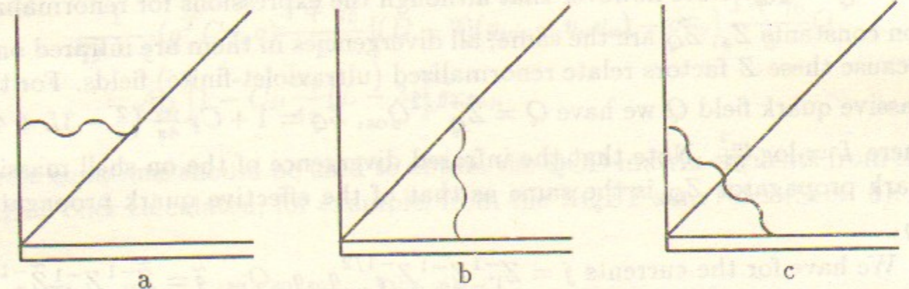
Figure 1: One-loop proper vertex
