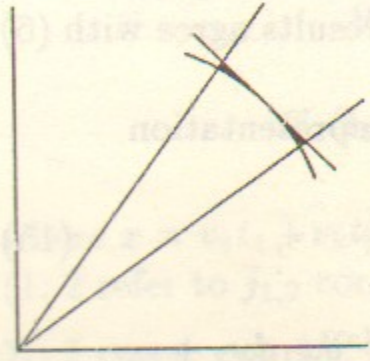
Figure 6: Physical region of double spectral densities
