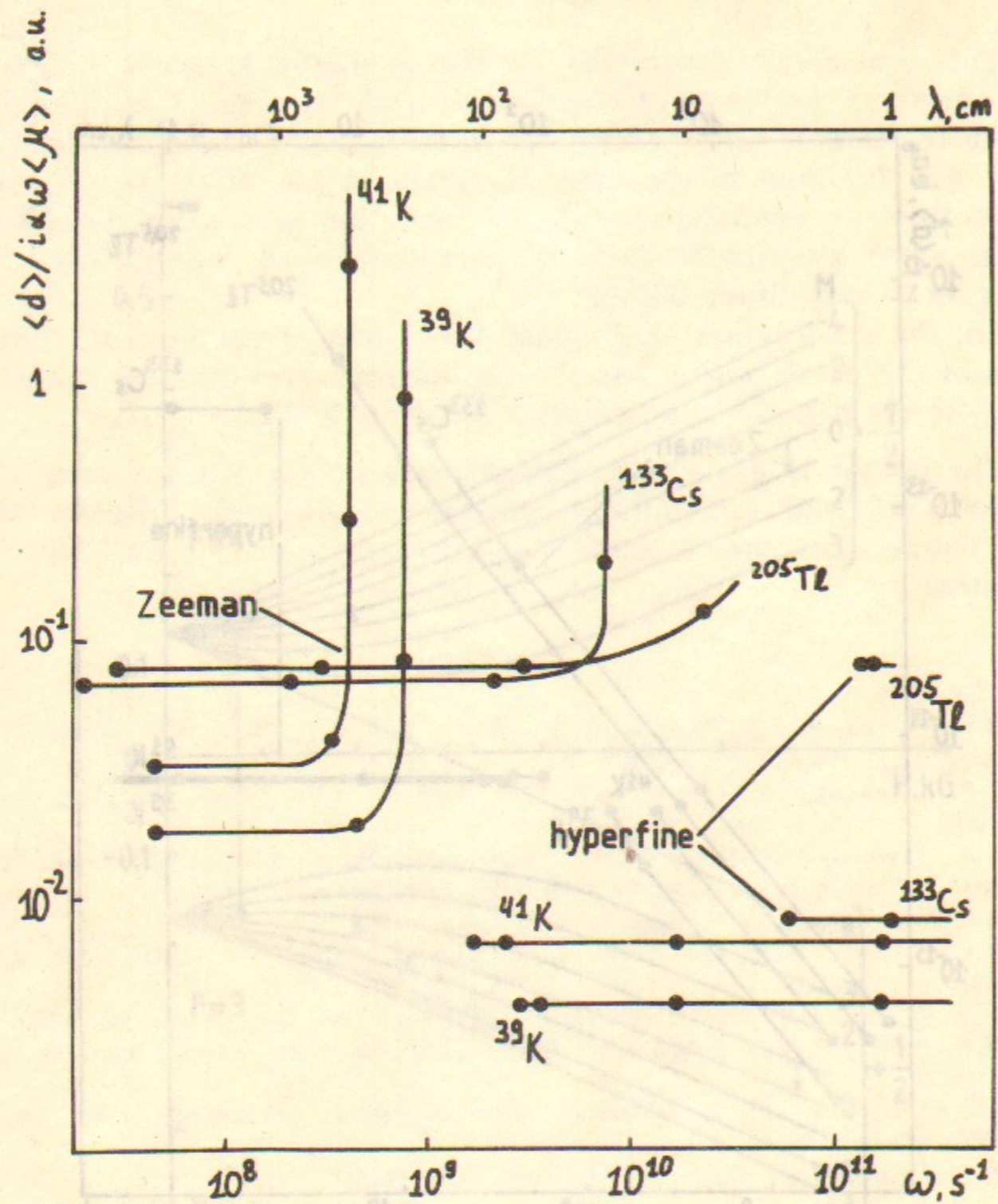
Fig. 3. The parameters of the ratio of the useful signal to the background as a functions of the external magnetic field and transition frequency. Notations like at Fig. 2.
