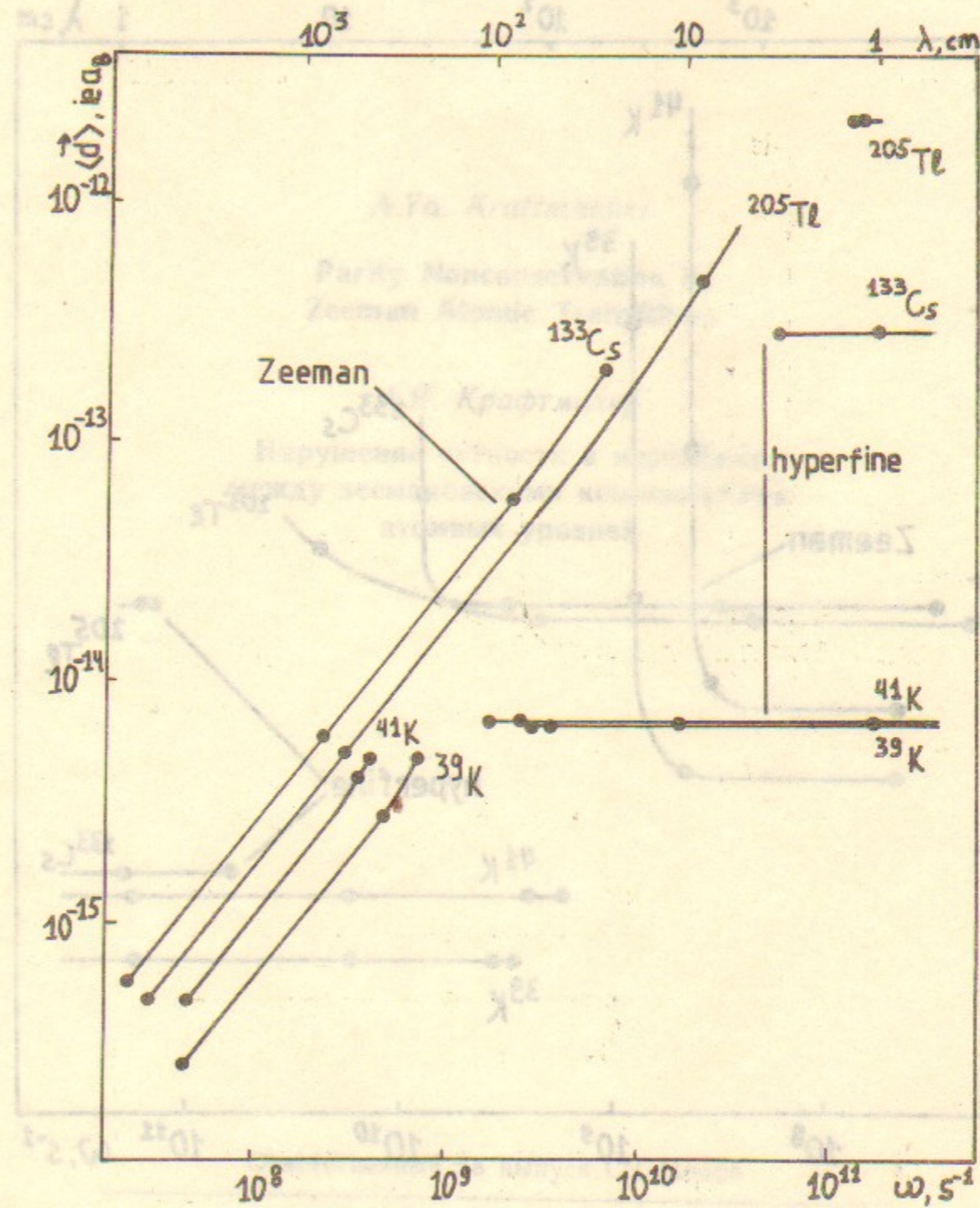
Fig. 2. P-odd E1-transition amplitudes between the Zeeman and hyperfine terms of different atoms as a functions of the external field and transition frequency. The points on the curves correspond to the values of magnetic field (from left to right and from down to up) 0, (for hyperfine transitions) or 10 G (for Zeeman ones), 100 G, 1 kG, 10 kG.
