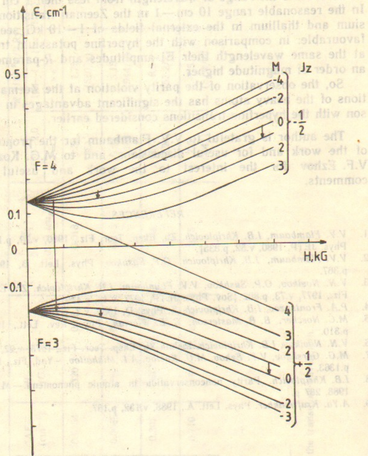
Fig. 1. Zeeman splitting of the hyperfine terms of ^{133}\text{Cs} 6s level as a function of external field. H_c = 1640 G—the scale of the field.
